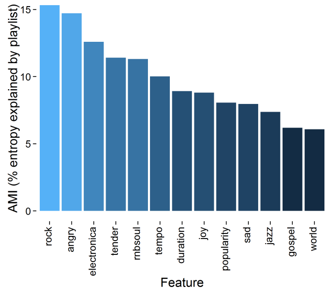
Figure 3. Features are ranked by their Adjusted Mutual Information with playlist membership. Playlists are distinguished more by whether they contain ROCK or ANGRY music than by whether they contain POPULAR or WORLD.
